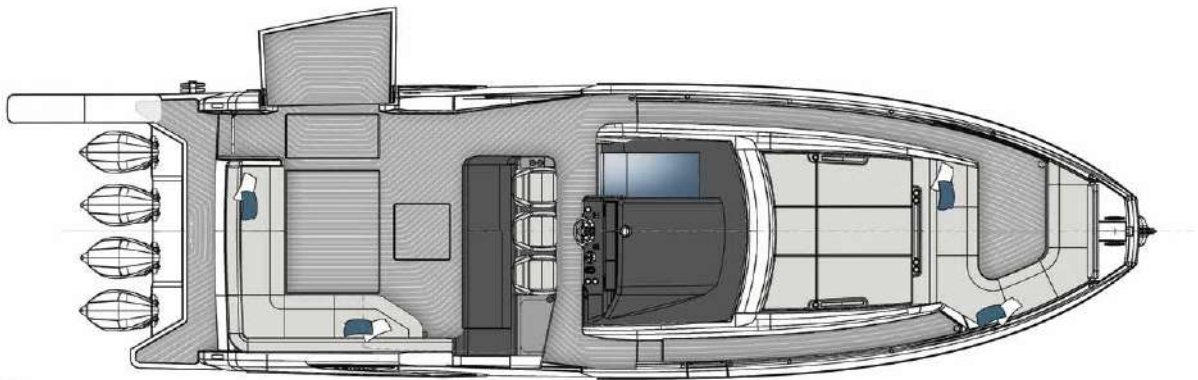
MAIN DECK
